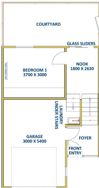
Ground Level +
