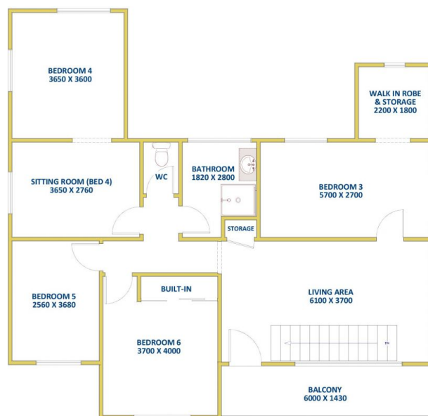
FIRST LEVEL
