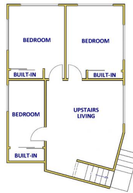
UPPER LEVEL
